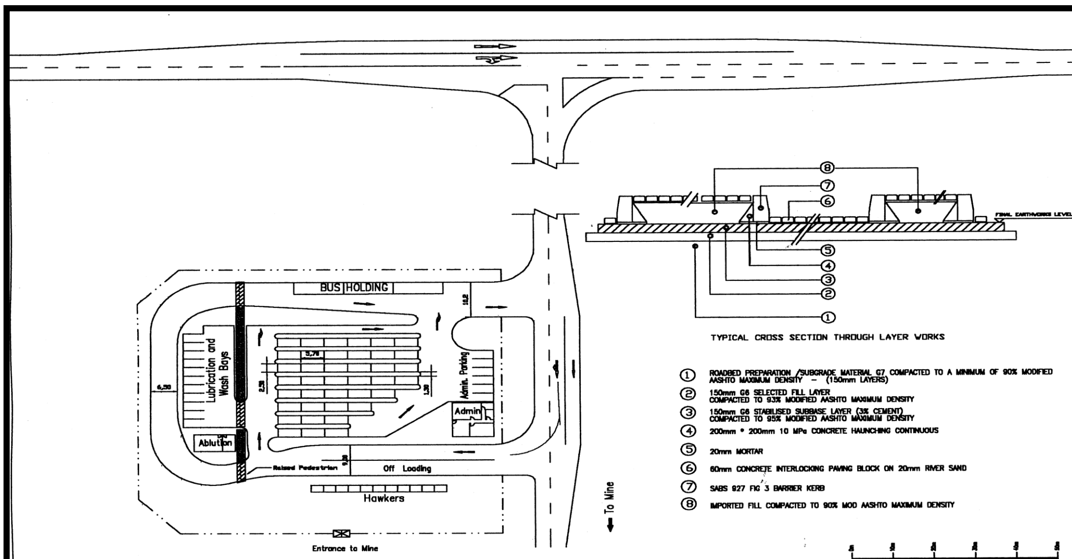
PROPOSED TAXI LAYOUT FIGURE 3.2
